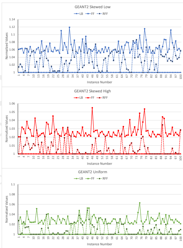
Fig. 6. Normalized solutions to 300 problem instances, GEANT2
