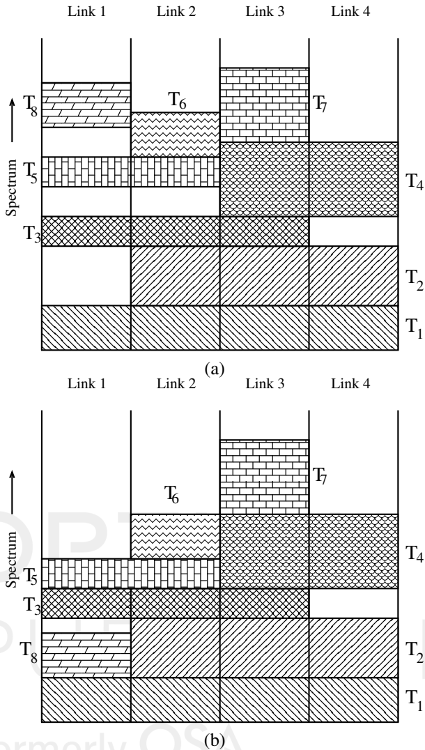
Fig. 1. Proof of the FF optimality property: (a) initial optimal solution, (b) modified optimal solution
