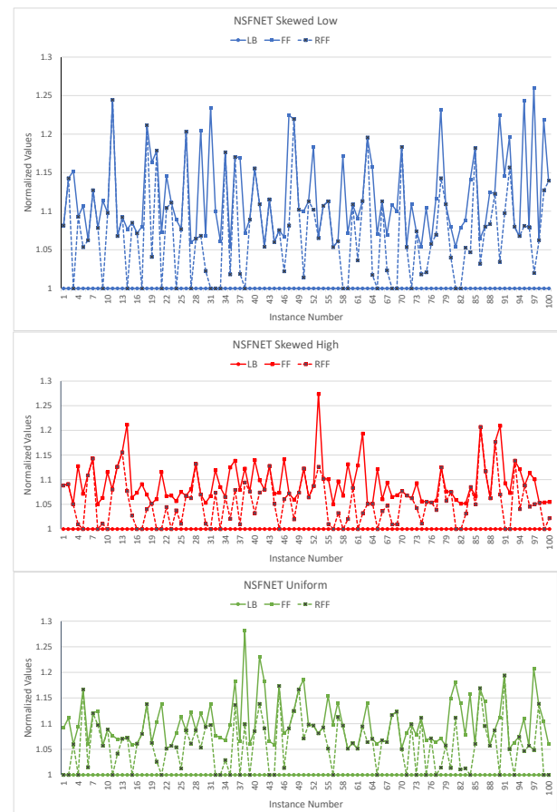
Fig. 5. Normalized solutions to 300 problem instances, NSFNET
