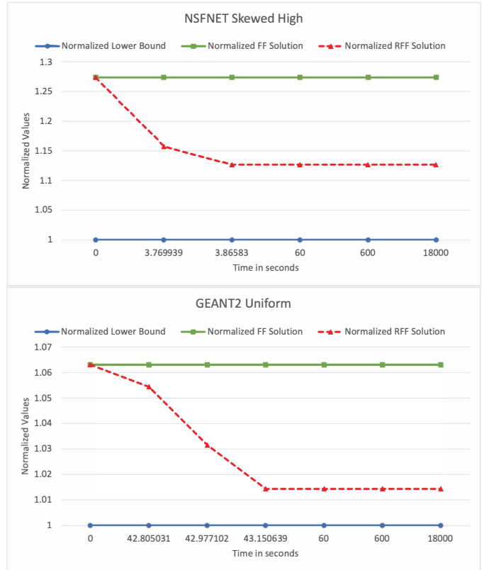
Fig. 3. Improvement of RFF solution vs. time, no parallelism (single-thread execution); time axis not in linear scale
